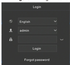
Figure 4-2 Login interface
